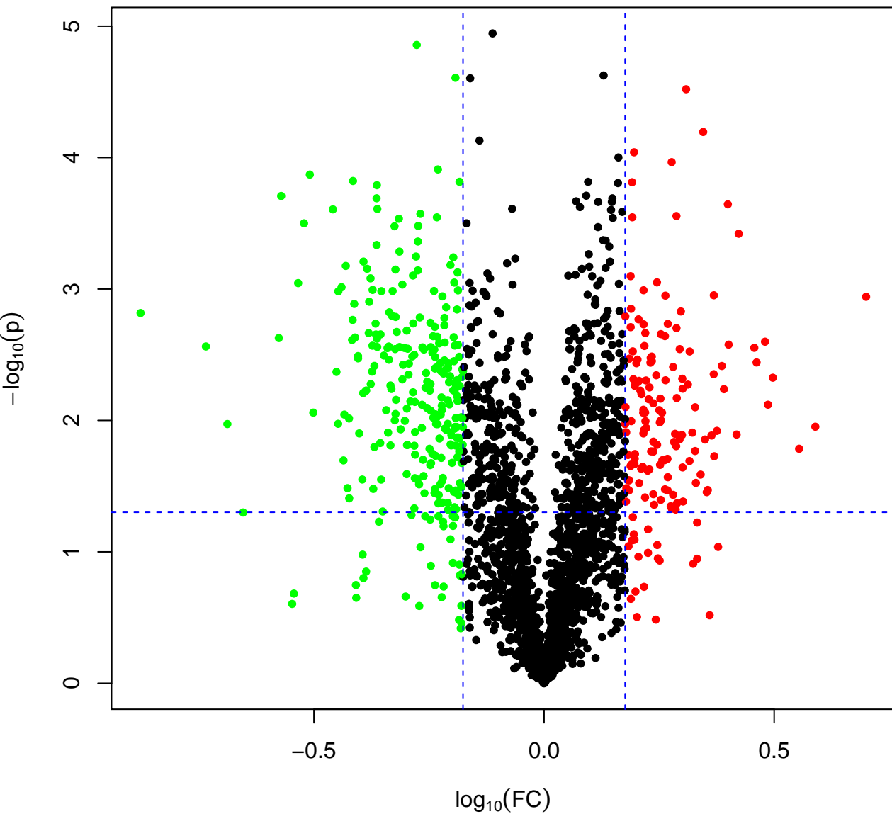
Volcano plot
